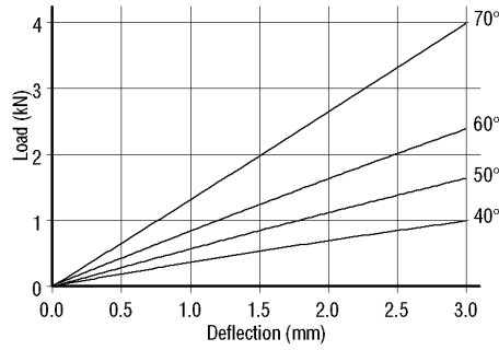
Compression Characteristics
