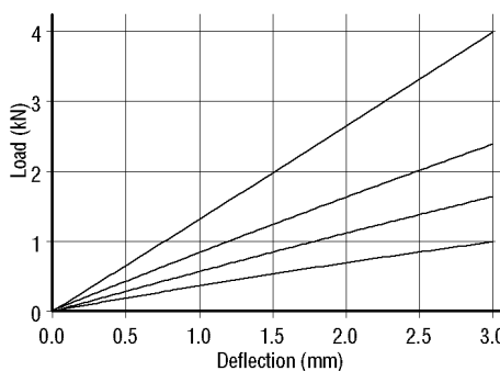
Compression Characteristics
