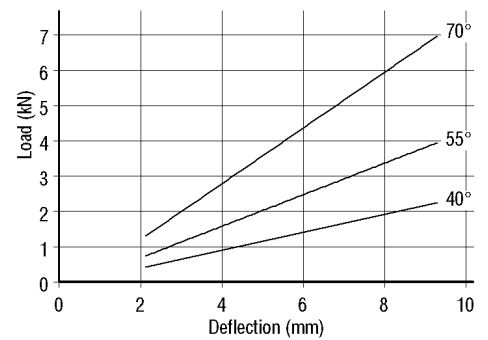
Compression Characteristics
