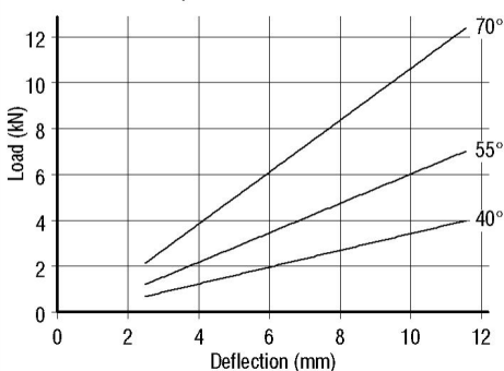
Compression Characteristics
