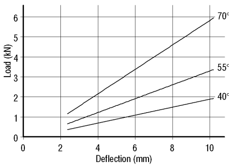
Compression Characteristics
