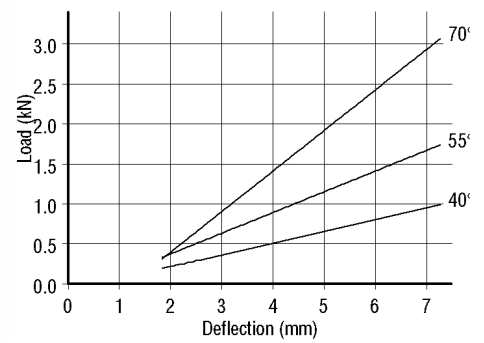
Compression Characteristics
