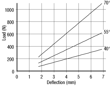
Compression Characteristics
