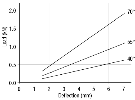
Compression Characteristics
