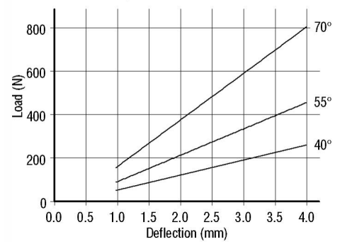
Compression Characteristics
