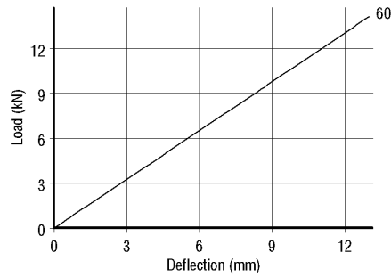
Compression Characteristics
