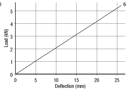
Shear Characteristics
