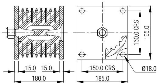
Part No. SIDE-MTG1207
