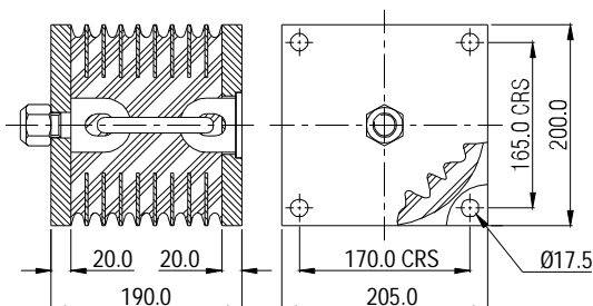
Part No. SIDE-MTG1208
