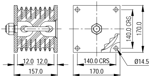
Part No. SIDE-MTG1199
